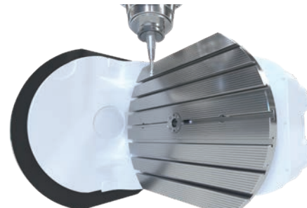
2-axis swivel rotary table of VM 500 U
